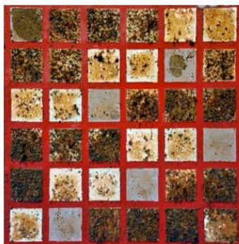
Maritime fouling on samples Source: Fraunhofer IFAM
