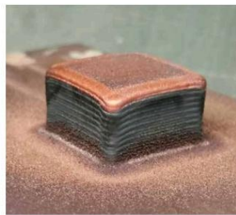
Build up: pure copper bulk material
