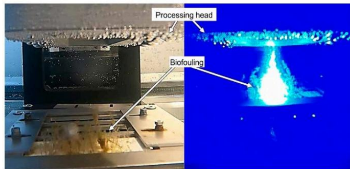
Underwater laser process in side view: Laser off (left) and on (right) Source: LZH
